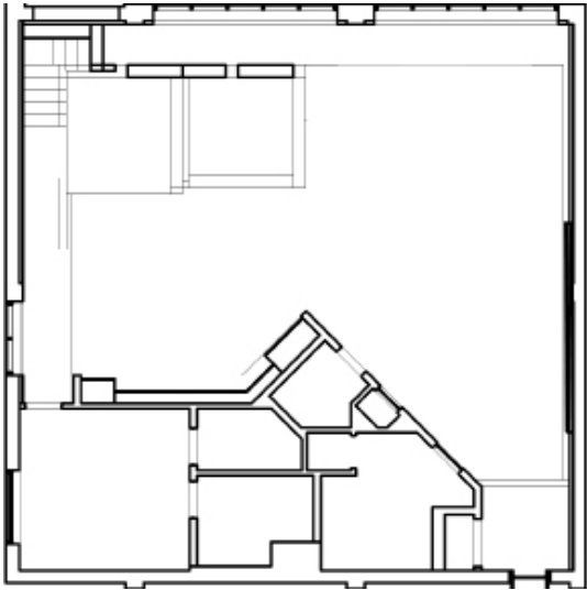
REFLECTED CEILING PLAN: LEVEL ONE SCALE: 1/8"=1'-0"
