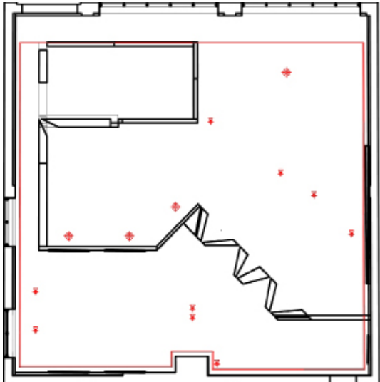
REFLECTED CEILING PLAN: LEVEL TWO SCALE: 1/8"=1'-0"
